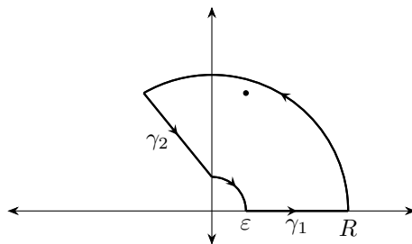
Figure 7: The contour \Gamma_{R,\varepsilon} containing a single pole of f .
